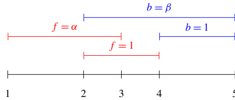
Fig. 3. Example of fuzzy interval model and algebra. In non-shown intervals all propositional letters are evaluated to 0.
