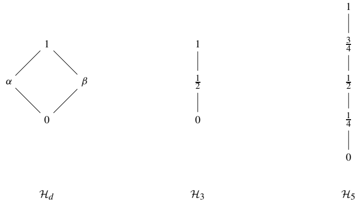
Fig. 2. Graphical representation of three Heyting algebras used in this paper.
